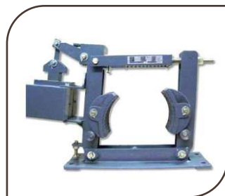
Magnetic Brake
